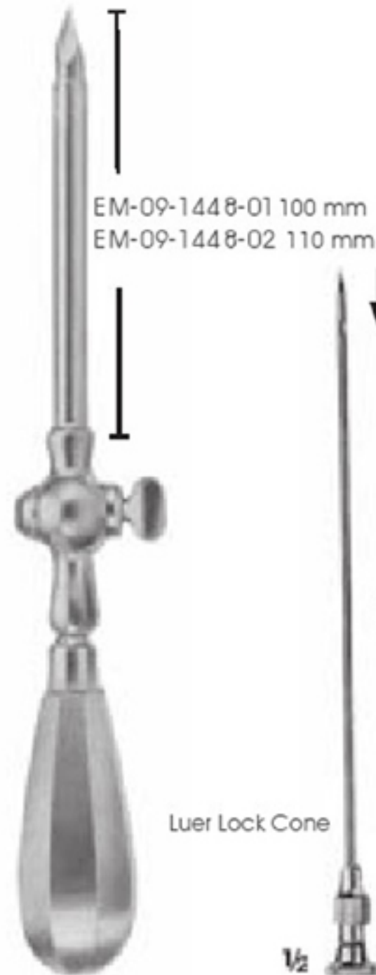
BUELAU EM-09-1448-01 EM-09-1448-02 Empyema trokar Inside Outside EM-09-1448-01 Ø 6.5 mm Ø 8.0 mm EM-09-1448-02 Ø 9.0 mm Ø 10.0 mm
